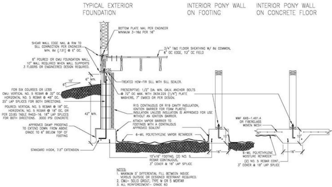
16 17 23.85. Figure R403-25 Typical foundation and footing details.
